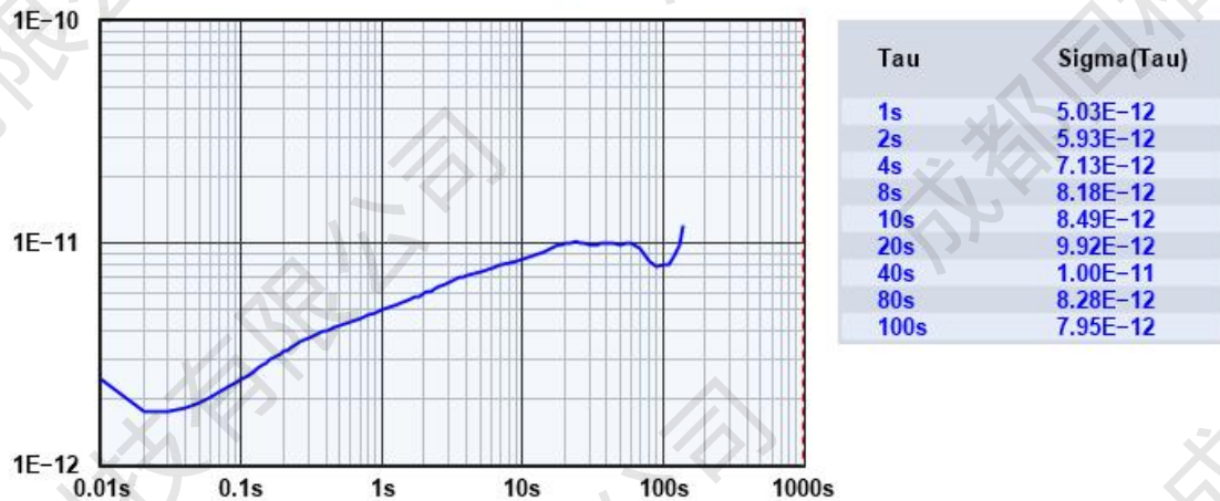
Allan Deviation \sigma_y(\tau)
